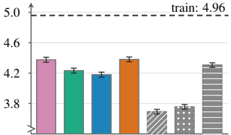
(c) HPSv3
