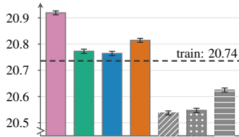
(a) PickScore
